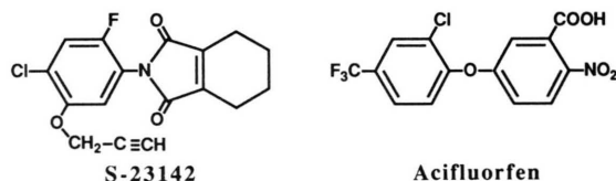
Fig. 1. Chemical structure of S-23142 and acifluorfen (AF).
